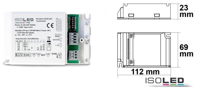
111989 | LED MULTI transformer 12V/24V/350mA/500mA/700mA, Push + 1-10V dimmable, SELV Compatible with LED Daylight Sensor 112619
