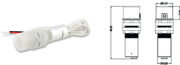
112619 | Daylight sensor passive for parallel connection in active 1-10V control signal lines Compatible with LED Multi Transformer 111989
