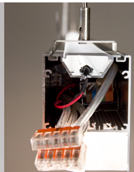
LED luminaire profile UP&DOWN1 (113483) with wire suspension and built-in SYS-ONE transformer (113521) and antenna led out.
